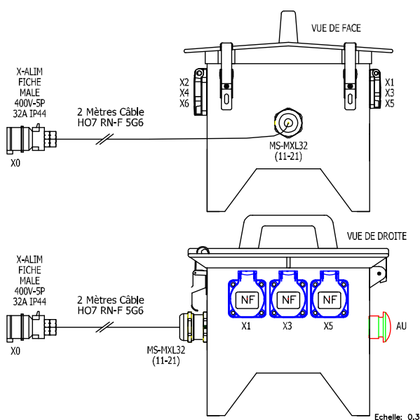
Coffret XR16M, Caoutchouc Dimensions 320x320x320mm (LxHxP)
